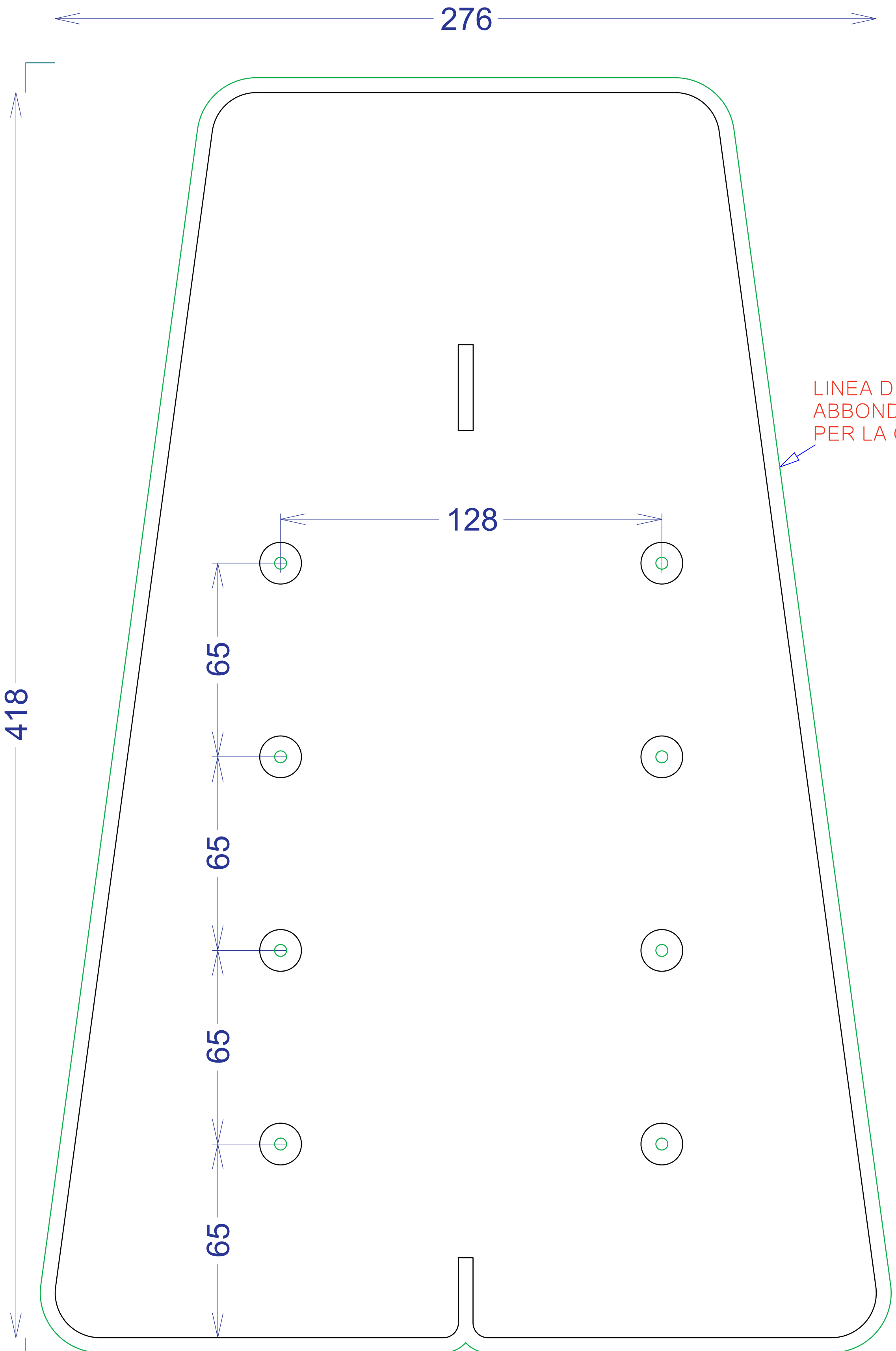
PINZA LATO STAMPA COD. 300_303_3048-00_DIS1
