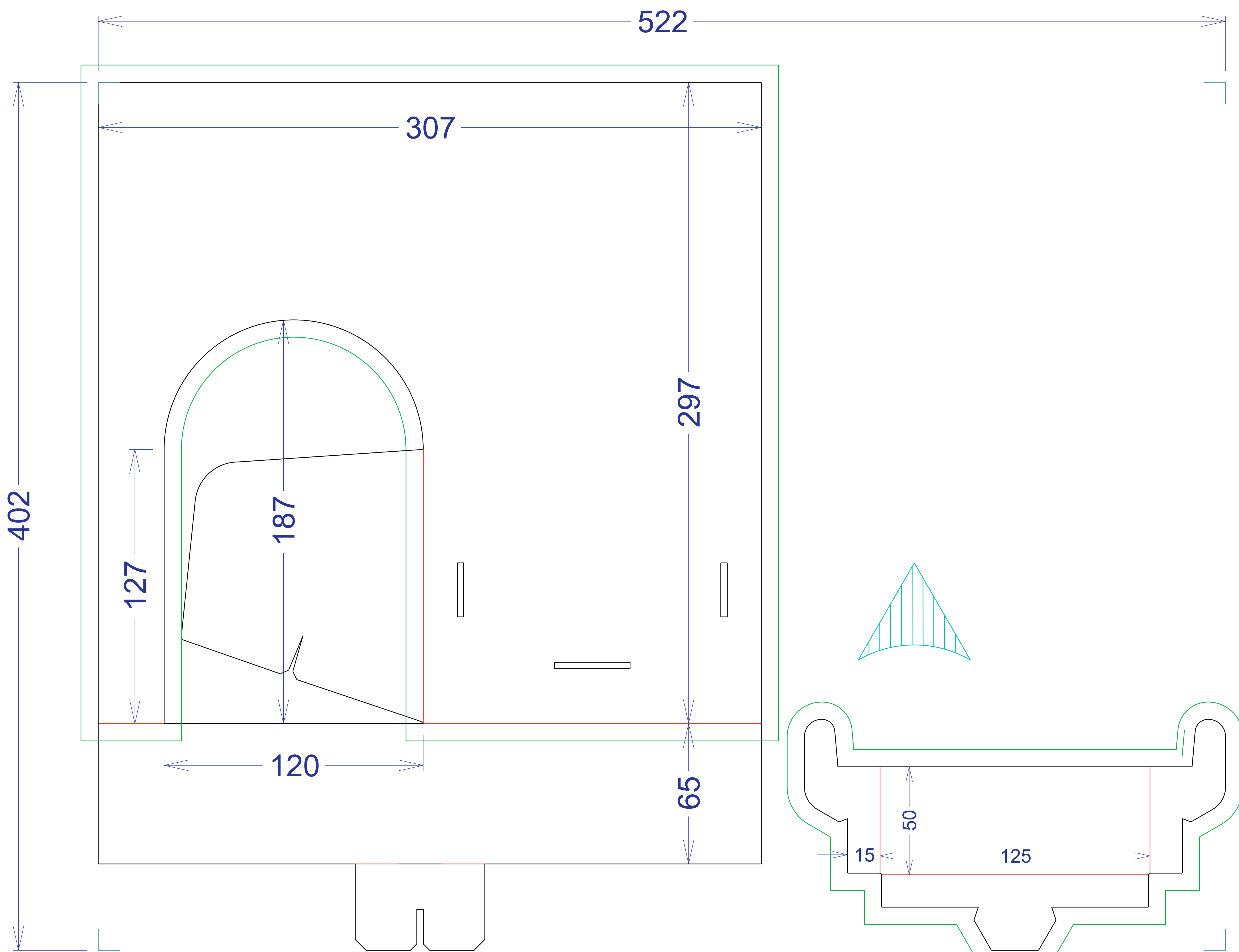
PINZA LATO STAMPA COD. 800_3002-02_DIS1
