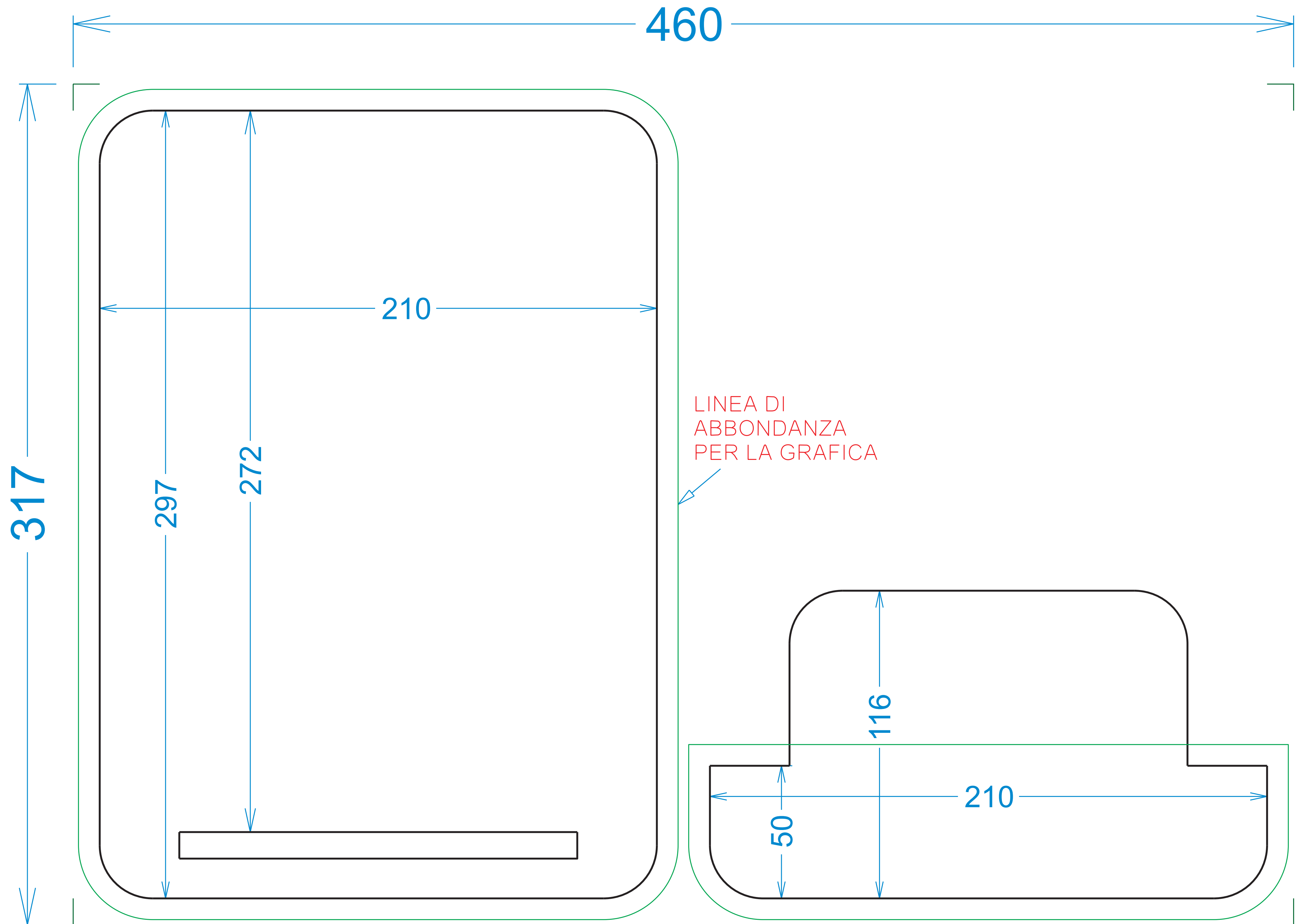
PINZA LATO STAMPA COD. 800_3107-00_DIS1
