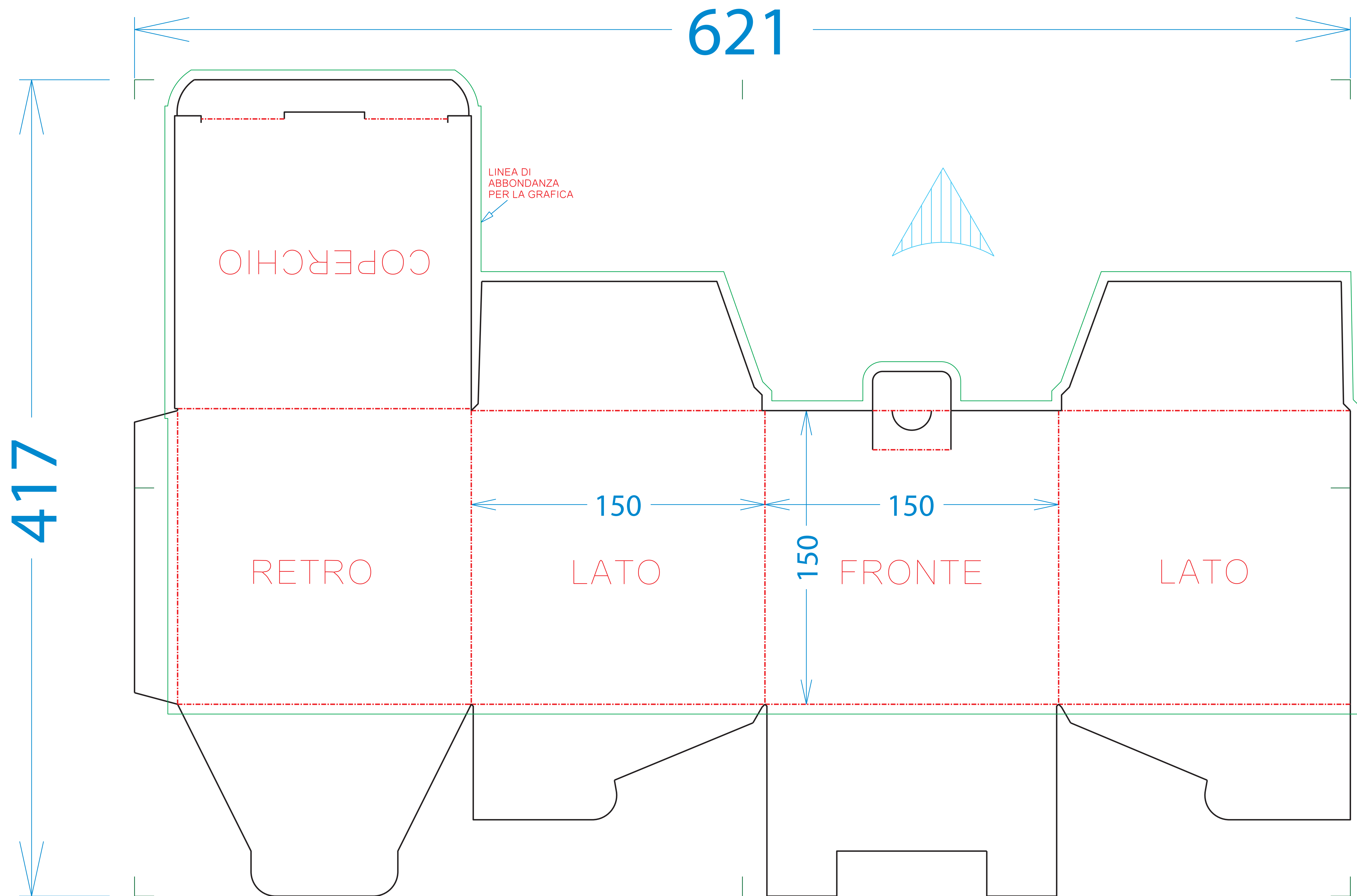
PINZA LATO STAMPA COD. 800_5002-00_DIS1
