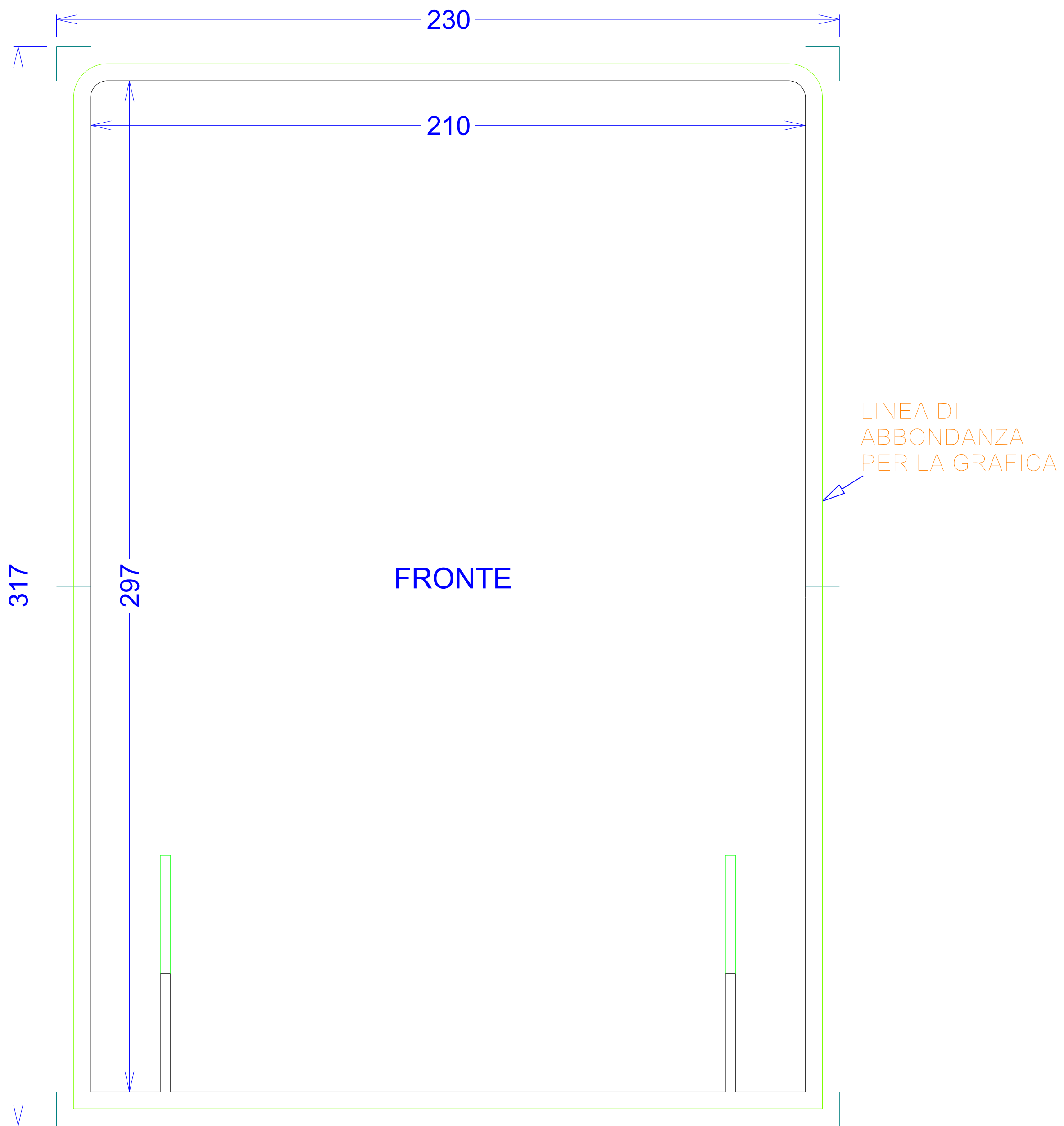
PINZA LATO STAMPA COD. 300_302_3044-00_DIS11
